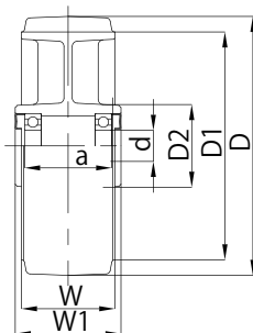
HB200x90
