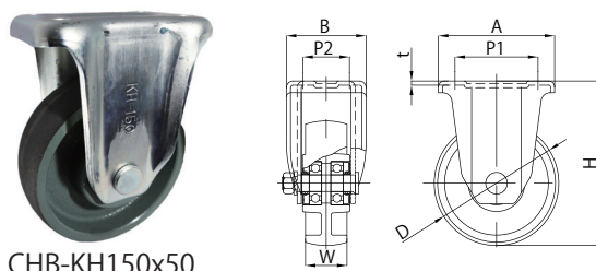
CHB-KH150x50
