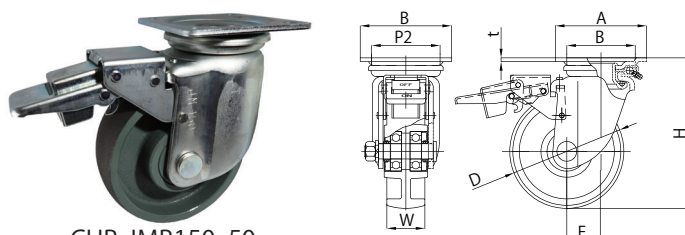
CHB-JMB150x50
